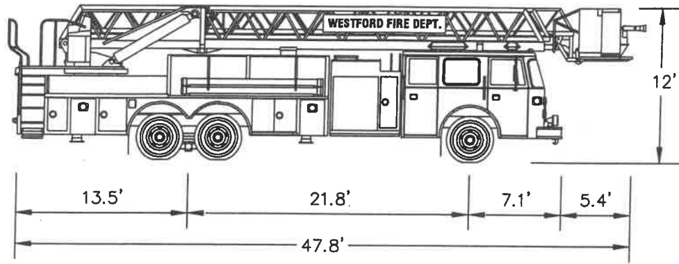
WESTFORD TOWER LADDER APPARATUS
